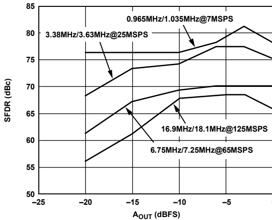
Figure 48. Dual-Tone SFDR vs. A_{OUT} @ f_{OUT} = f_{CLK}/7
