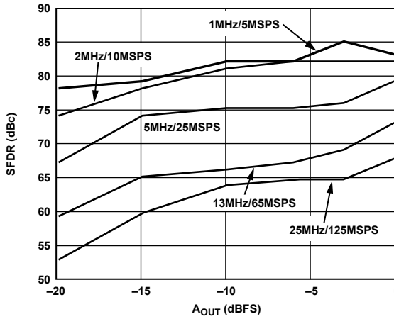
Figure 47. Single-Tone SFDR vs. A_{OUT} @ f_{OUT} = f_{CLK}/5
