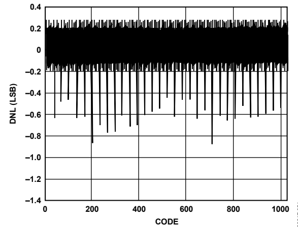
Figure 51. Typical DNL
