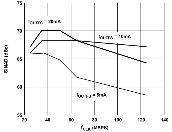
Figure 32. SINAD vs. f_{CLK} and I_{OUTFS} @ f_{OUT} = 5 MHz and 0 dBFS
