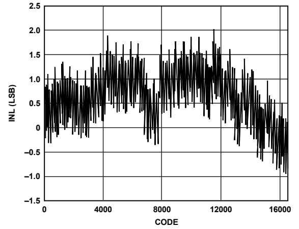
Figure 50. Typical INL
