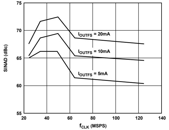
Figure 49. SINAD vs. f_{CLK} and I_{OUTFS} @ f_{OUT} = 5 MHz and 0 dBFS
