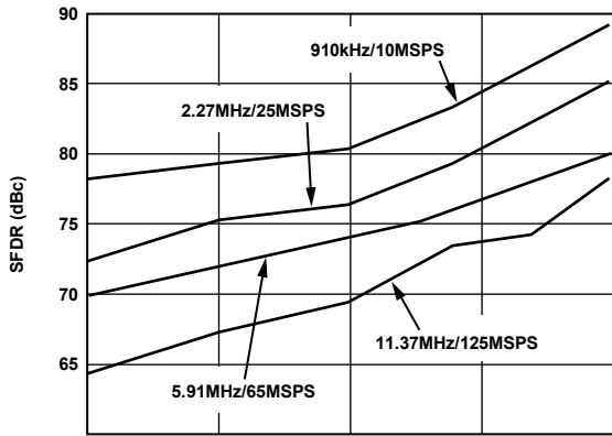
Figure 46. Single-Tone SFDR vs. A_{OUT} @ f_{OUT} = f_{CLK}/11
