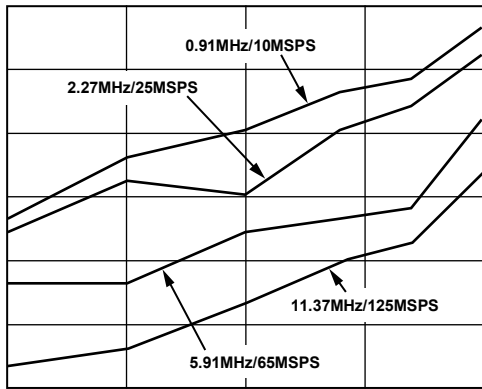
Figure 29. Single-Tone SFDR vs. A_{OUT} @ f_{OUT} = f_{CLK}/11
