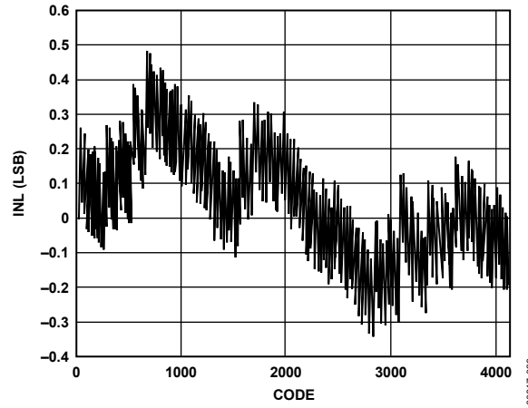
Figure 33. Typical INL
