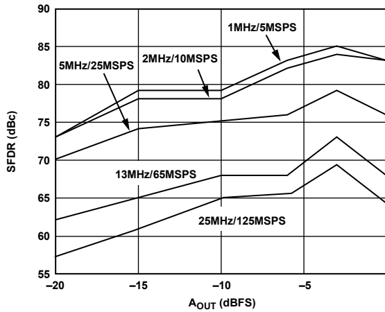
Figure 30. Single-Tone SFDR vs. A_{OUT} @ f_{OUT} = f_{CLK}/5
