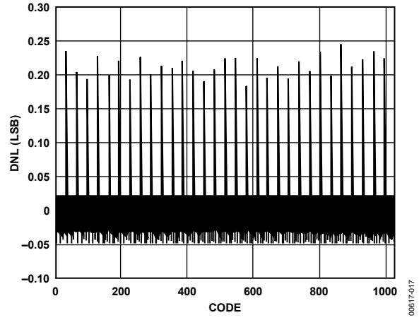
Figure 17. Typical DNL
