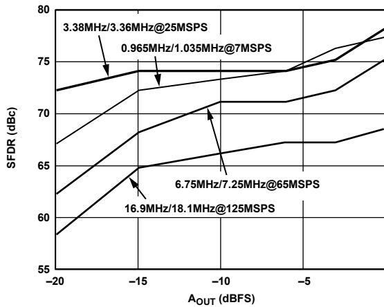
Figure 31. Dual-Tone SFDR vs. A_{OUT} @ f_{OUT} = f_{CLK}/7
